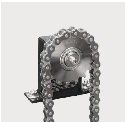
SPANN-BOX® size 1 (type KL) with sprocket
